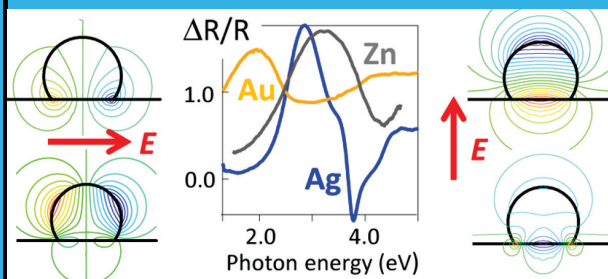
Fig: Differential reflectivity spectra for various metal on alumina and simulated absorption modes
